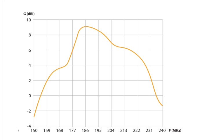
FREQUENCY RESPONSE
