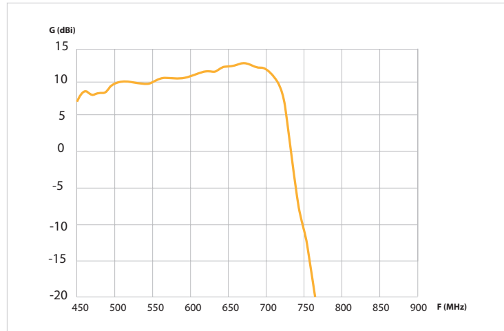
FREQUENCY RESPONSE
